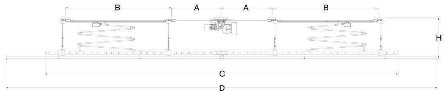
Quick lock connection for easy and fast installation.
