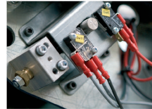
All safety micro-switches integrated into motor unit.
